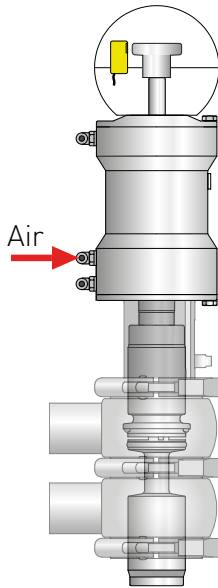
Valve open
